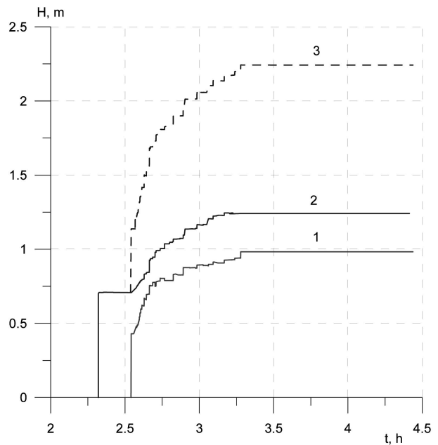
Fig. 7. Pool Depth and Layer Thicknesses (1 - Oxides; 2 - Steel; 3 - Pool Depth)
