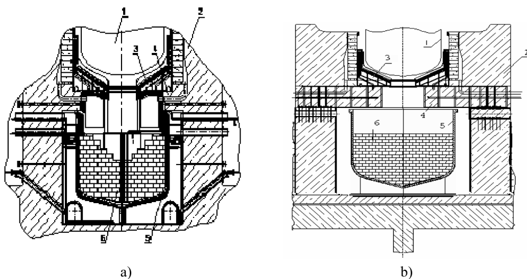
Fig. 1. Principal Layout of Core Catcher of Tyanwan (a) and Kudankulam NPPs (b) (1 - Reactor Pressure Vessel (RPV); 2 - Reactor Cavity; 3 - Lower Plate; 4 - Cantilever Girder; 5 - Core Catcher Vessel; 6 - SM)
