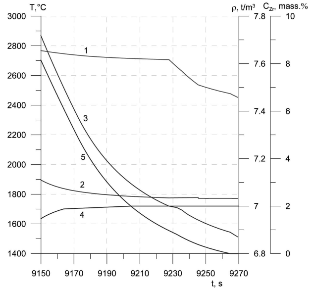
Fig. 6. Evolution of Melt Parameters in the Beginning of the Second Relocation Stage (1 - Temperature of Oxidic Melt; 2 - Temperature of Steel Melt; 3 - Density of Oxidic Melt; 4 - Density of Steel Melt; 5 - Zr Concentration in Oxidic Melt)
